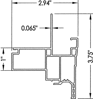
1 FRAME HEAD
