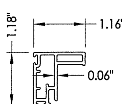
2 SASH STILE/RAIL
