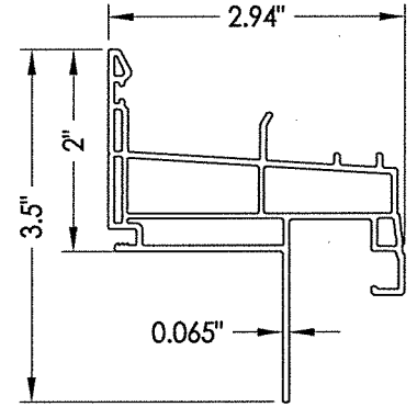
6 SILL
