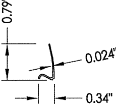
7 GLAZING BEAD
